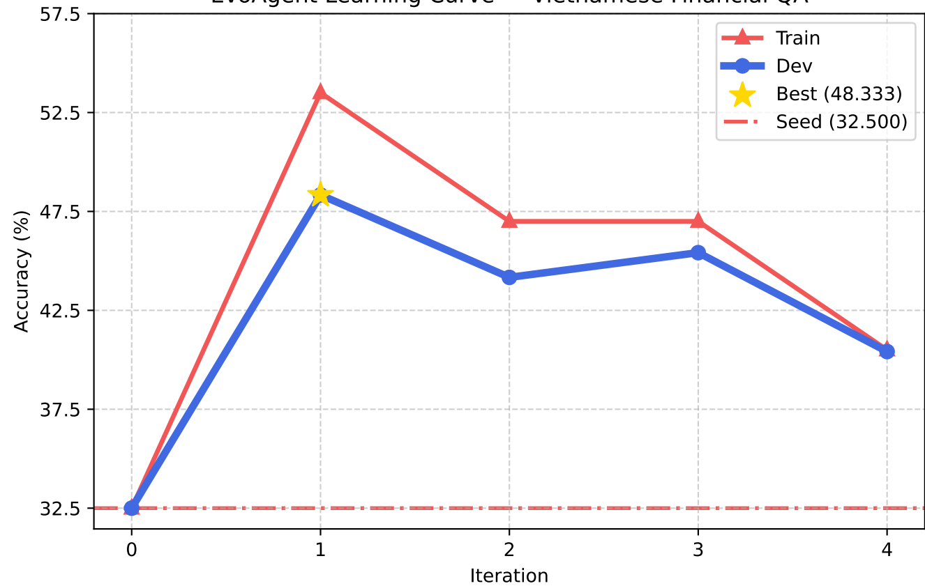
EvoAgent Learning Curve — Vietnamese Financial QA
